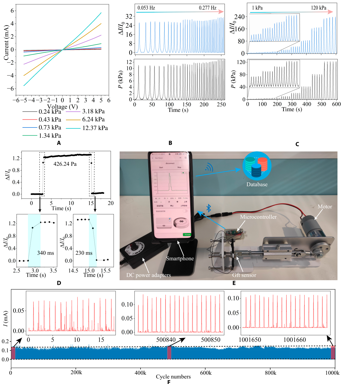
Fig. 3. Sensor actual use performance test. (A) Current–voltage curves of the Gft sensor under various pressures. (B) Current response of the Gft sensor at an external force of 10 kPa; the frequency increases from 0.053 to 0.277 Hz. (C) The current response of the Gft sensor under external force increases from 1 to 120 kPa. (D) Response and recovery time of the Gft sensor under the pressure of 426.24 Pa. (E) Wireless cyclic sensing performance test system. (F) Stability and reliability of the Gft sensor over 1 million cycles.
