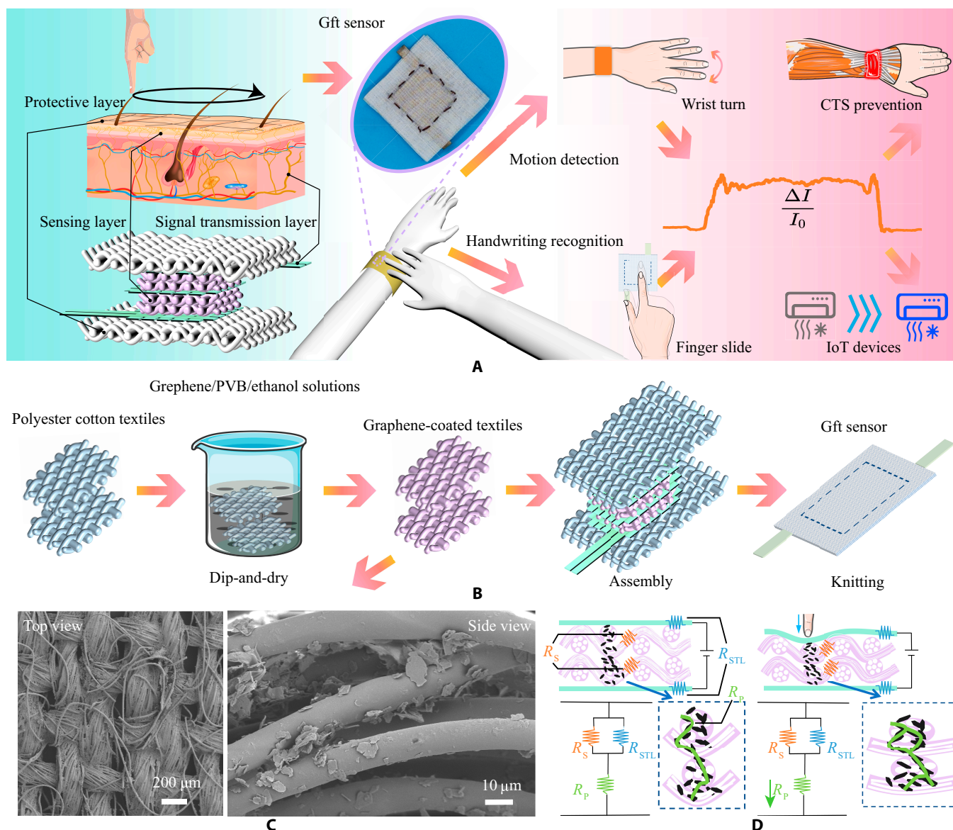
Fig. 1. Sensing principle and practical applications. (A) Structure and artificial intelligence applications of the skin-inspired Gft sensor. (B) Fabrication and assembly processes of the skin-inspired Gft sensor. (C) Scanning electron microscopy images of the top and side sections of the 4 wt% graphene/PVB-coated conductive fabric. (D) Analysis of the piezoresistive effect of the Gft sensor.
