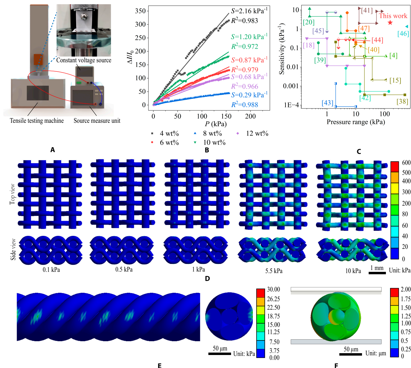
Fig. 2. Performance characterization of the Gft sensor. (A) Schematic diagram of an experimental device for tensile testing of the Gft sensor. (B) Performance comparison of Gft sensors manufactured by dip coating with different graphene concentrations. (C) Performance comparison between the Gft sensor and the reported full-textile pressure sensor. (D) Stress distribution of the sensing layer under different pressures. (E) Stress distribution and (F) deformation of a single fiber under compression (zoom in 5 times for display).
