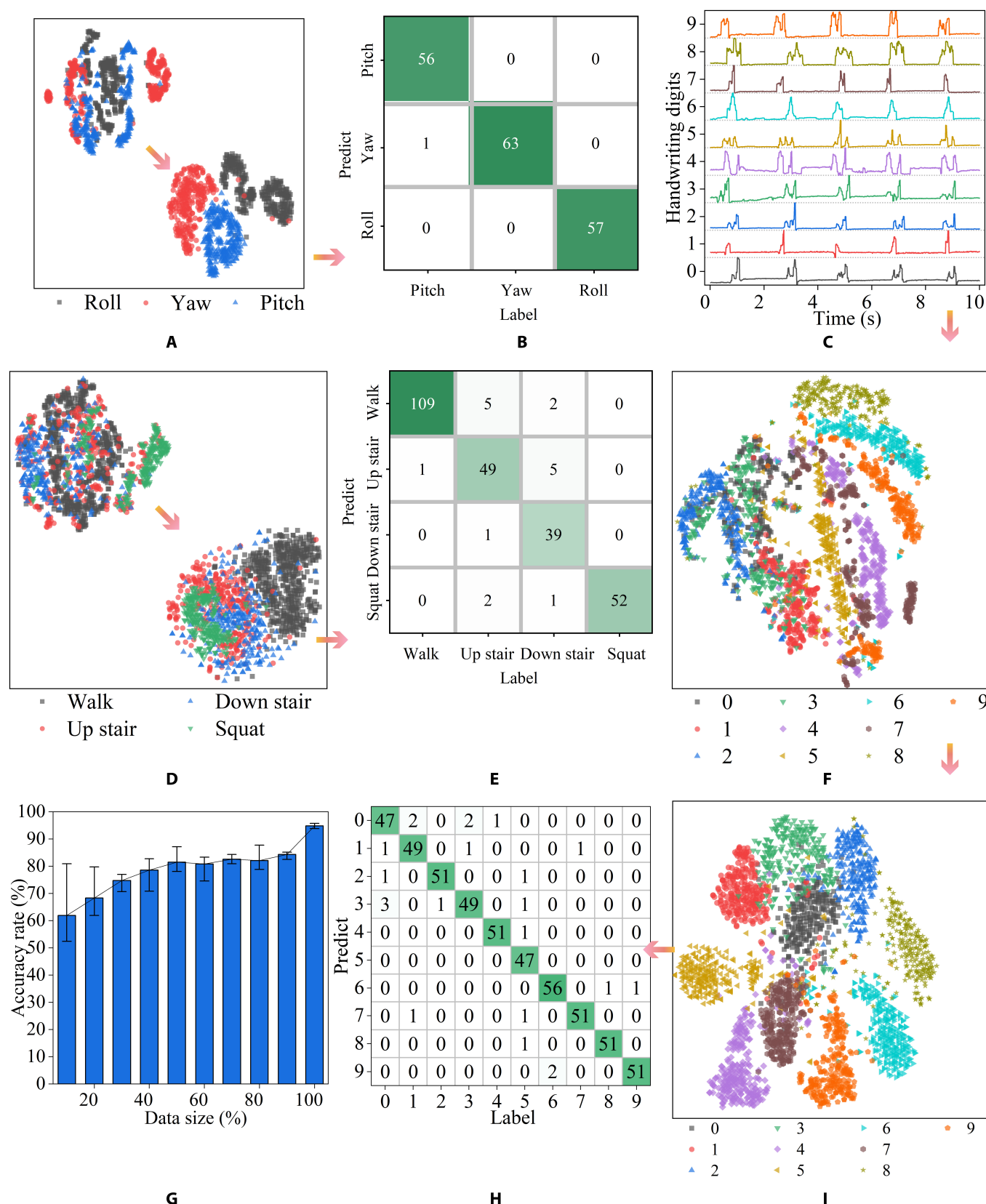
Fig. 5. Pattern recognition for complex tasks of sensors. (A) Dimension reduction visualization of the collected wrist rotation dataset and the features extracted by CNN t-SNE data. (B) Confusion matrix of the recognition results of wrist turn test set. (C) The 10-s response current curves of different handwritten digits. (D) t-SNE dimension reduction visualization of human activity dataset and its features. (E) Confusion matrix of the recognition results of human activity test set. (F) t-SNE dimension reduction output of handwritten digits on the wristband dataset. (G) Graph of recognition accuracy as training data increase. (H) Confusion matrix of the recognition results of the handwritten digit test set. (I) t-SNE dimension reduction visualization of the features of the handwritten digit dataset.
